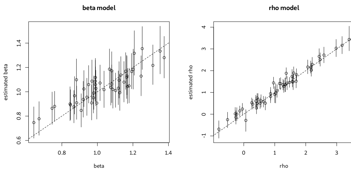
Figure C1: Parameter Recovery
