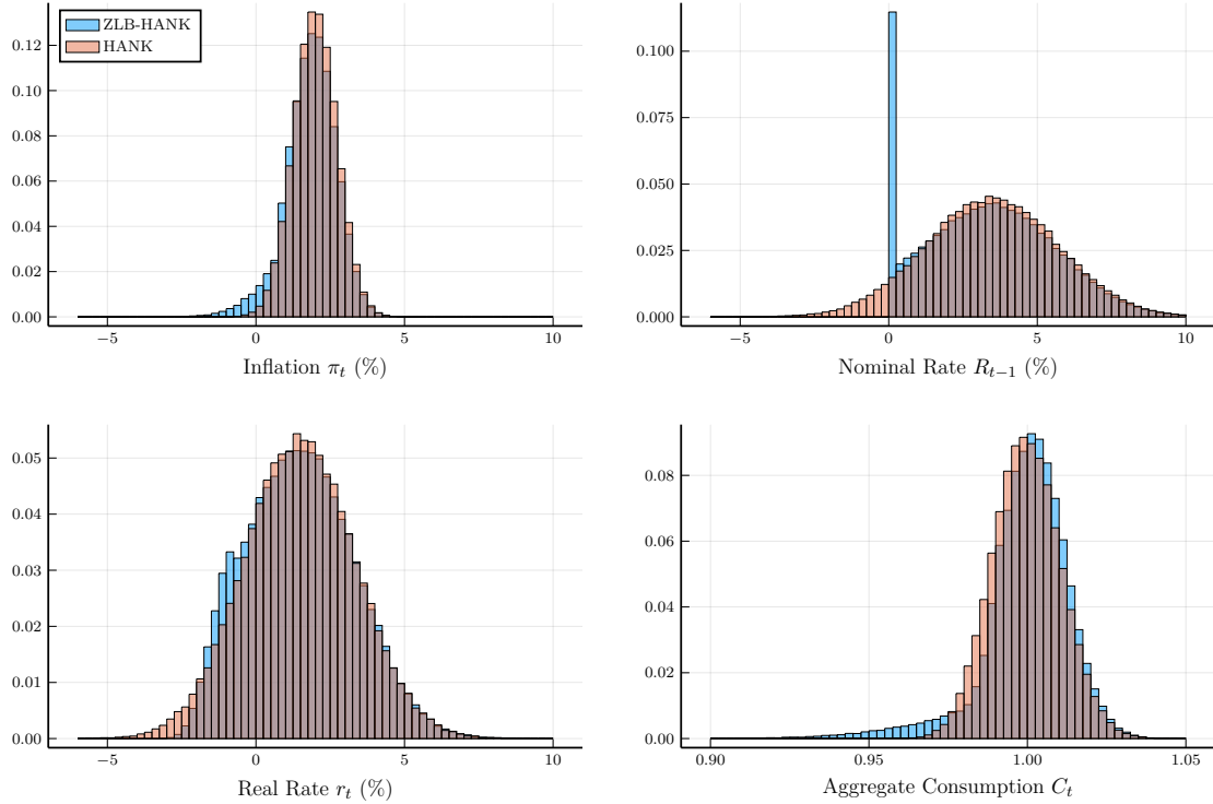
Figure 3: Ergodic Distributions.
