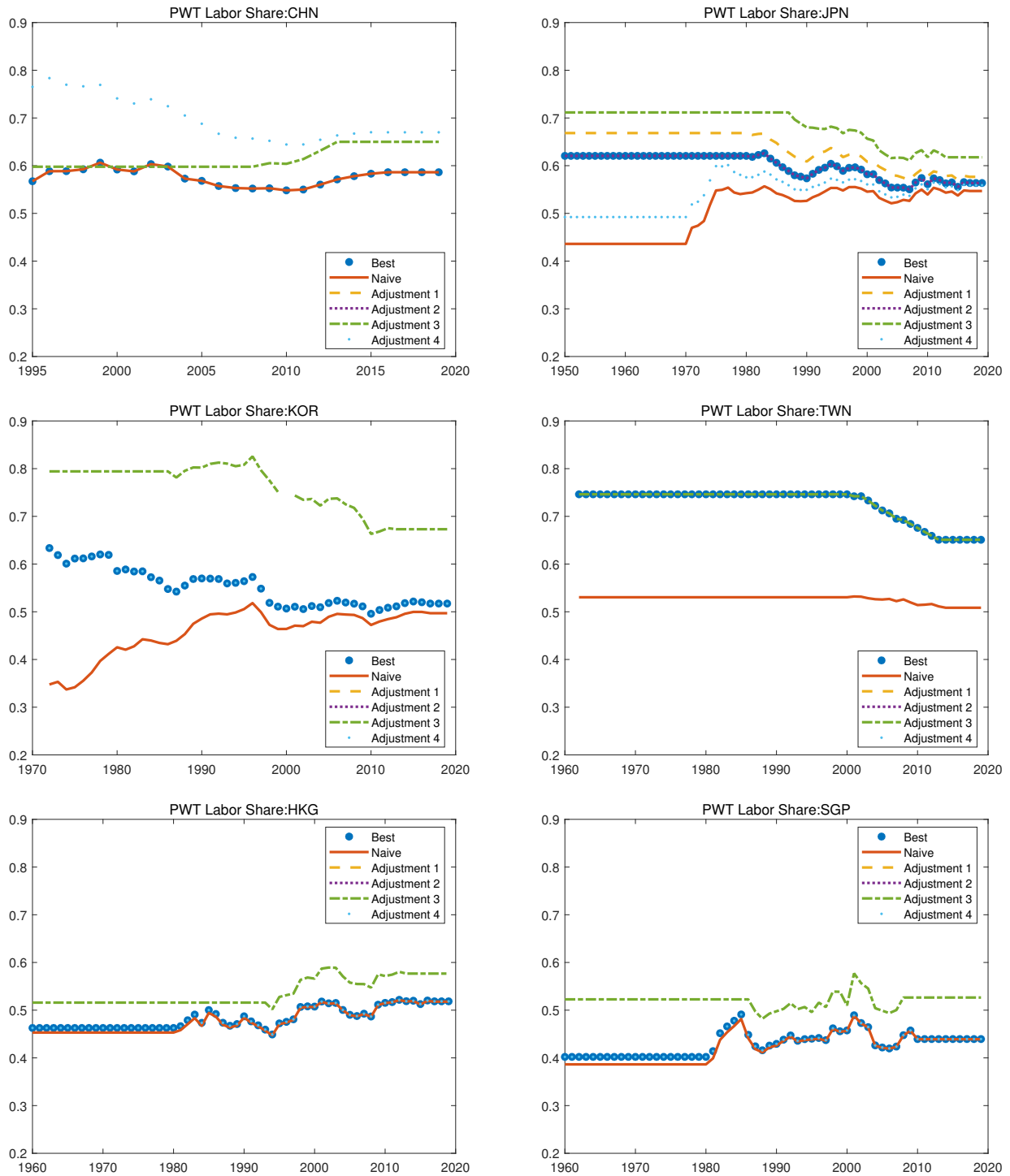
Figure D.1: Labor shares reported by PWT 10.0
