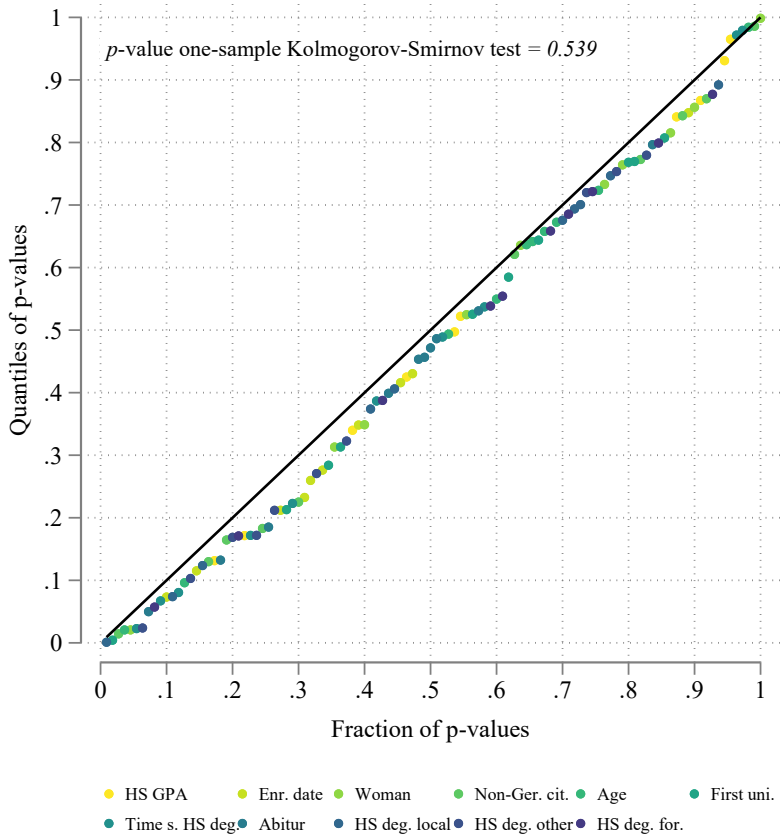
Figure 4: Quantile plot of p-values from regressing student characteristics on freshman orientation group dummies
