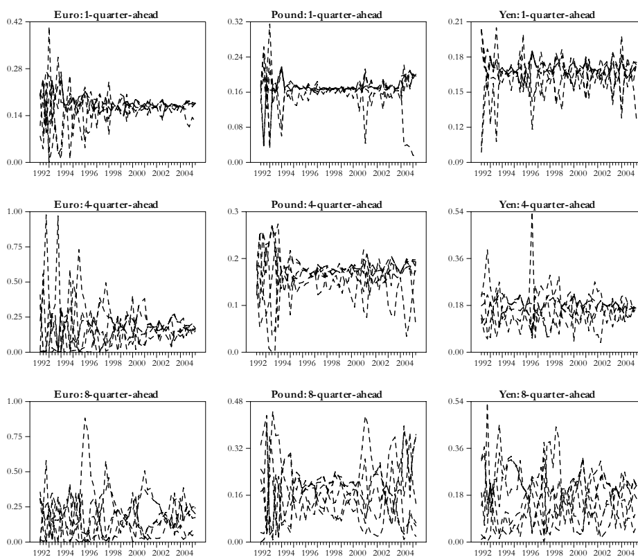
Figure 1: Weights used in Combining Forecasts
