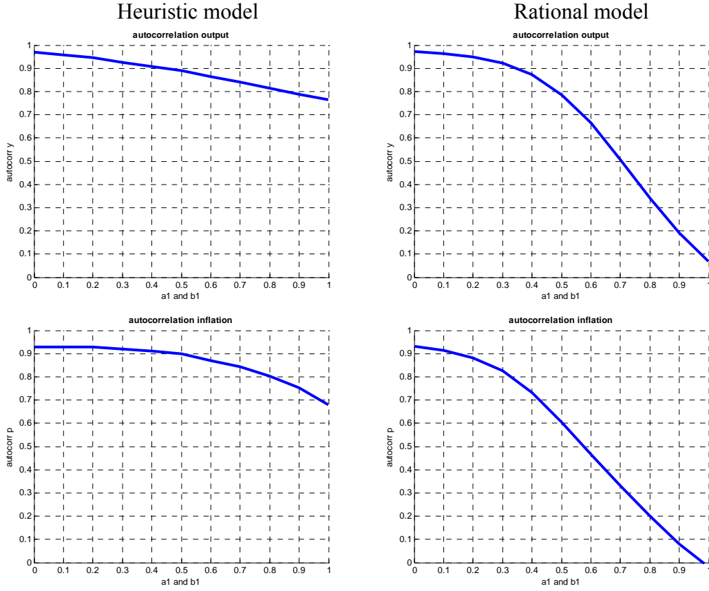
Figure 23: Autocorrelation coefficients of output gap and inflation
