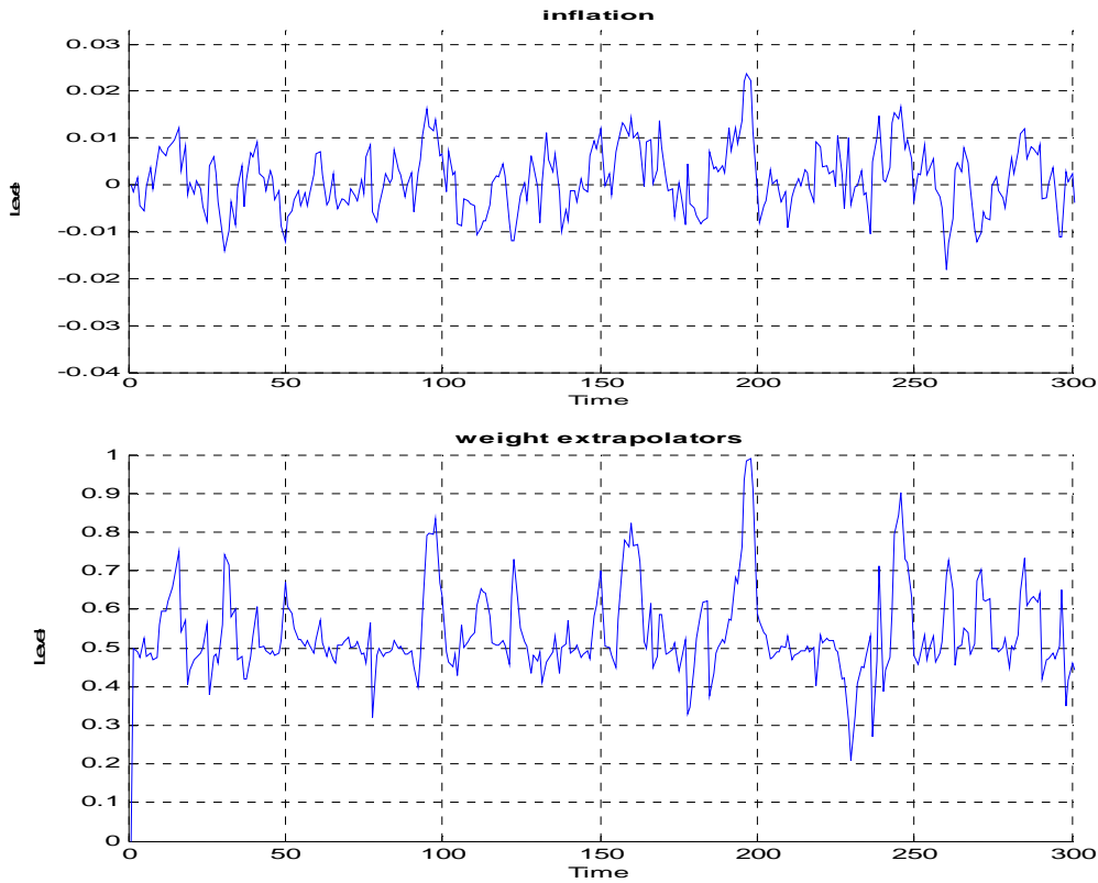
Figure 7: Inflation in the extended heuristic model with strict inflation targeting
