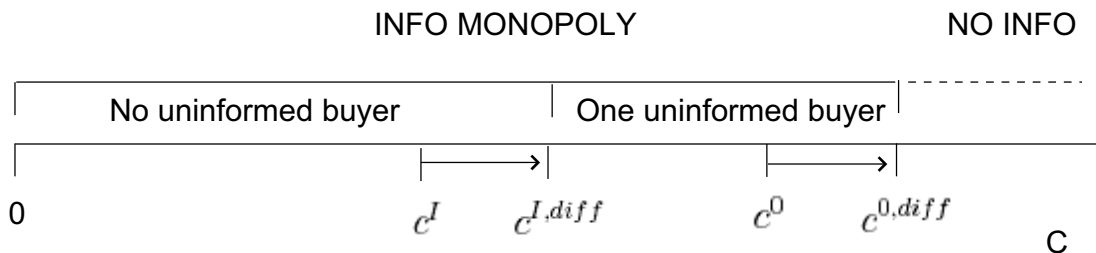
Figure 2: Equilibrium with heterogeneous messages
