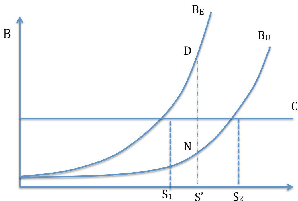
Figure 7: Good and bad equilibria
