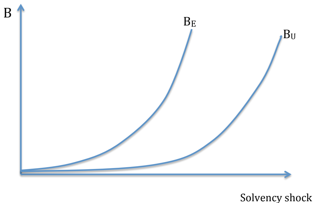
Figure 5: The benefits of default after a solvency shock
