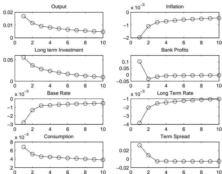
Figure 6: Productivity Shock
