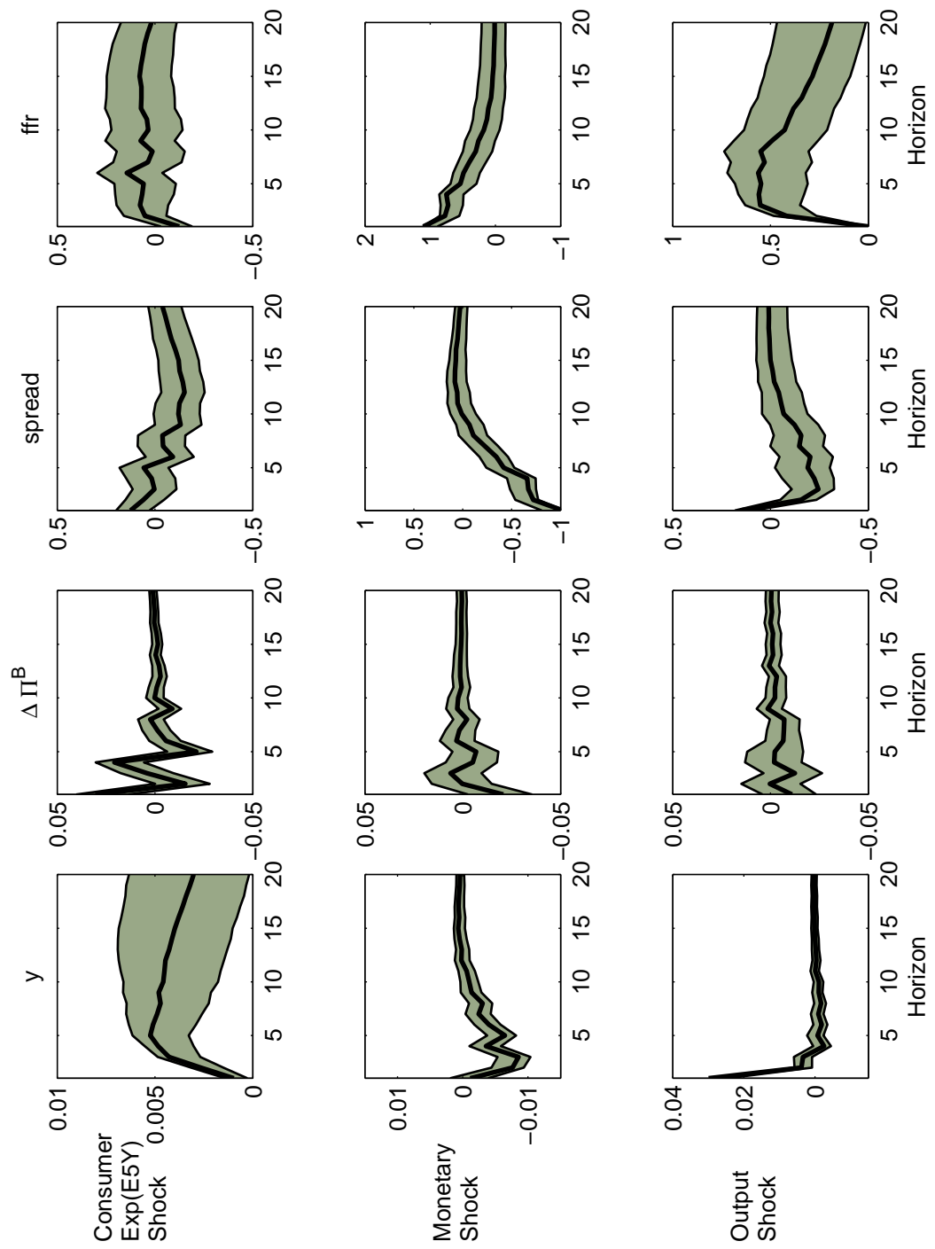
Figure 10: Impulse Responses
