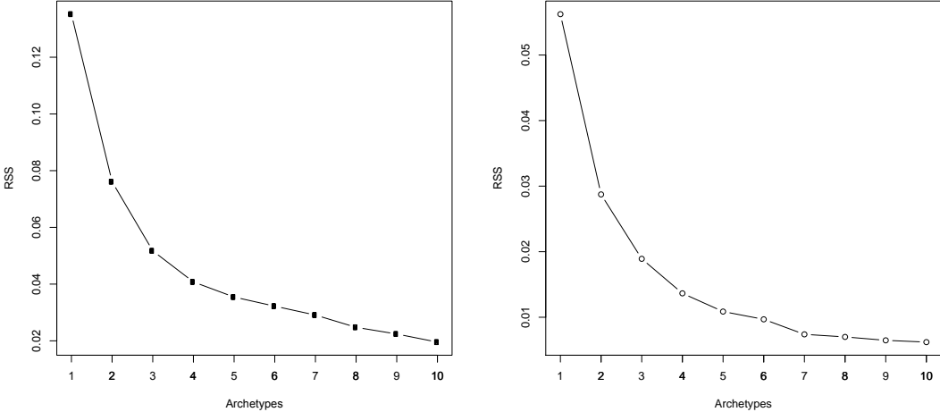
Figure 8: Screeplot for the top 1,500 economists with (left) and without (right) outliers
