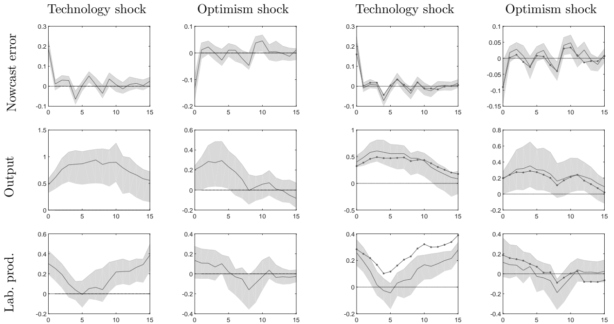
Figure 7: Impulse responses to technology and optimism shock under partial identification. Notes: Left panel shows results for weakly restricted nowcast error (alternative identification I); right panel shows results for identification based on sign restrictions. Solid lines display the median response for specification without long-run restriction on labor productivity; shaded areas indicate 68% highest-posterior-density intervals (alternative identification II). Solid lines with markers display the median response of specification without short-run restriction on nowcast error (alternative identification III). Horizontal axes measure quarters. Vertical axes: percentage points in case of nowcast error; percentage deviations from pre-shock level otherwise.
