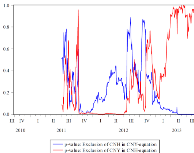
Figure 4. P-values of Rolling Block Exogeneity Test Statistics
