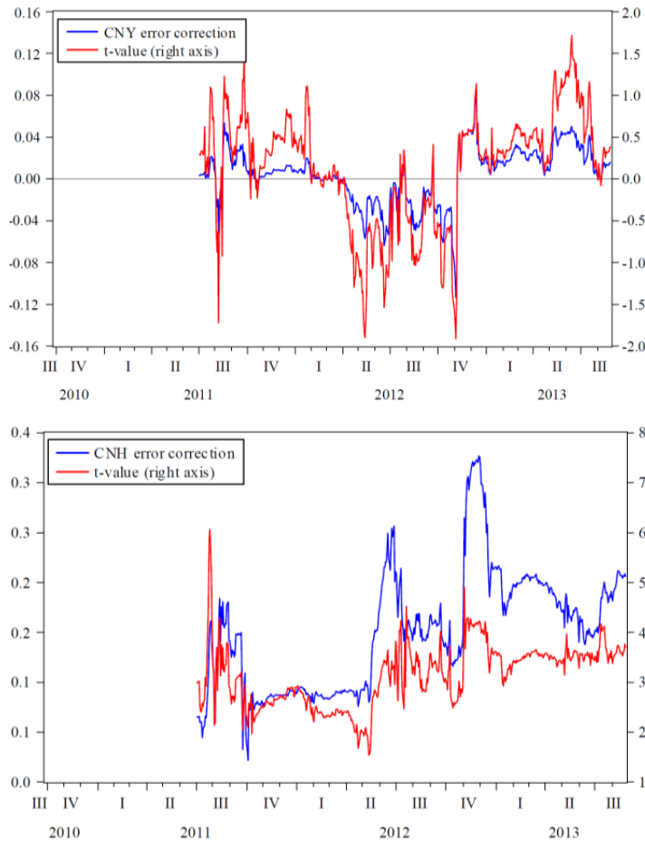
Figure 3. Rolling Estimates of Error-Correction Coefficient Estimates and their t-Statistics
