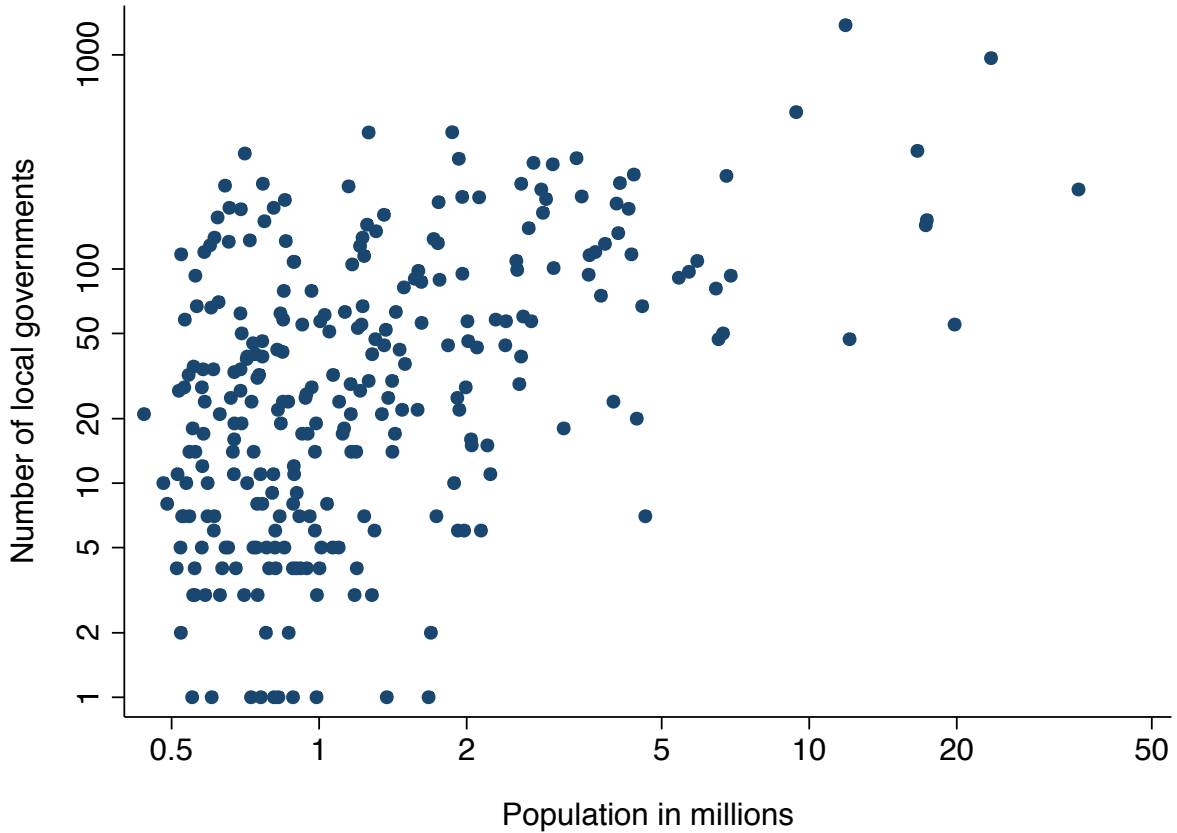
Figure 2: Number of municipalities and population across 275 cities in 28 OECD countries, 2012. Source: OECD (Regional Statistics).
