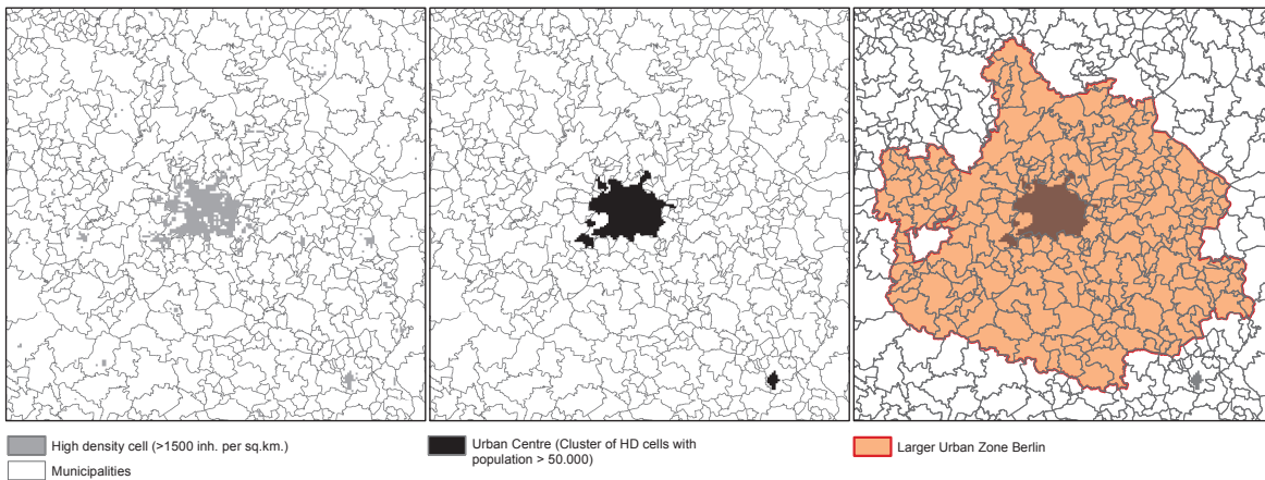
Figure 1: Construction of the Berlin functional urban area. Left panel shows the high-density cells with > 1500 inhabitants per square km and administrative municipal boundaries. Middle panel illustrates the construction of urban centers with total population > 50,000 . Right panel shows the construction of the larger urban zone based on bilateral commuting flows. Source: European Commission (prepared by DG Regional and Urban Policy).
