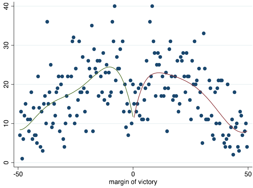
Figure A1. Density of the forcing variable
