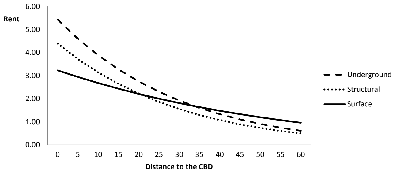
Figure 1: Equilibrium land rent when \tau = 0
