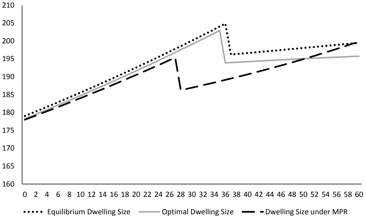
Fig. 3: Dwelling size when \tau = 0.2
