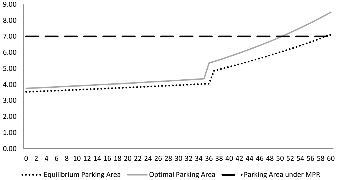
Fig. 2: Parking area when \tau = 0.2
