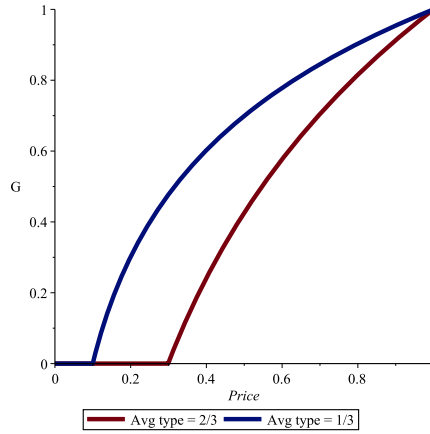
Figure 2: Price distributions H_{\frac{1}{3},1}^* and H_{\frac{2}{3},1}^* .
