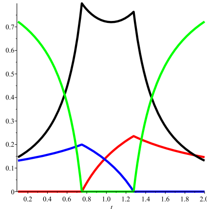
Figure 5: p_\tau(\tau) (black), p_\tau(\bar{\tau}) (red), p_\tau(\mu) (green) and p_\tau(\underline{\tau}) (blue)
