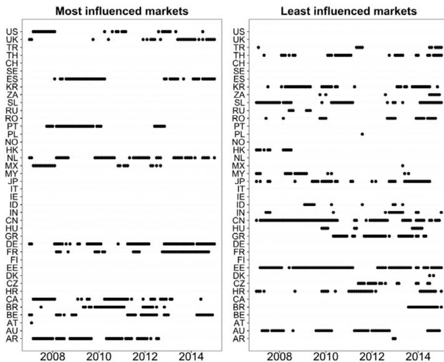
Figure 6. Top 3 markets with the highest in-degree \text{deg}^{\text{in}}(i) over all subsamples. Note: A point is drawn at the time t for three markets with the highest (left panel) or lowest (right panel) in-degree.
