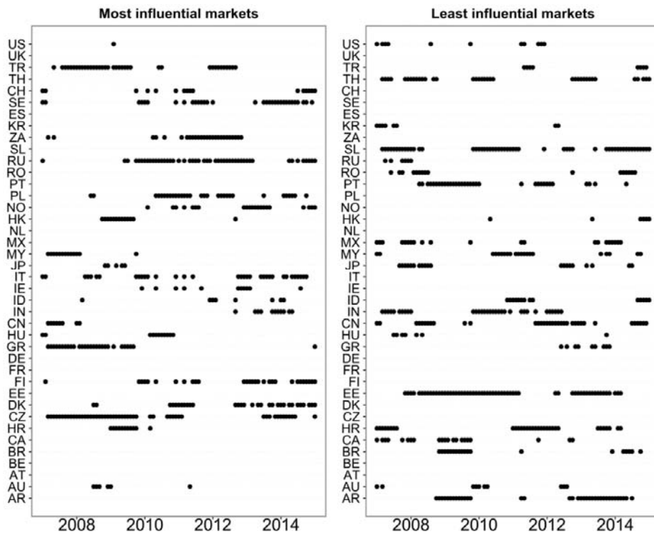
Figure 5. Top 3 markets with the highest out-degree \text{deg}^{\text{out}}(i) over all subsamples. Note: A point is drawn at time t for three markets with the highest (left panel) or lowest (right panel) out-degree.
