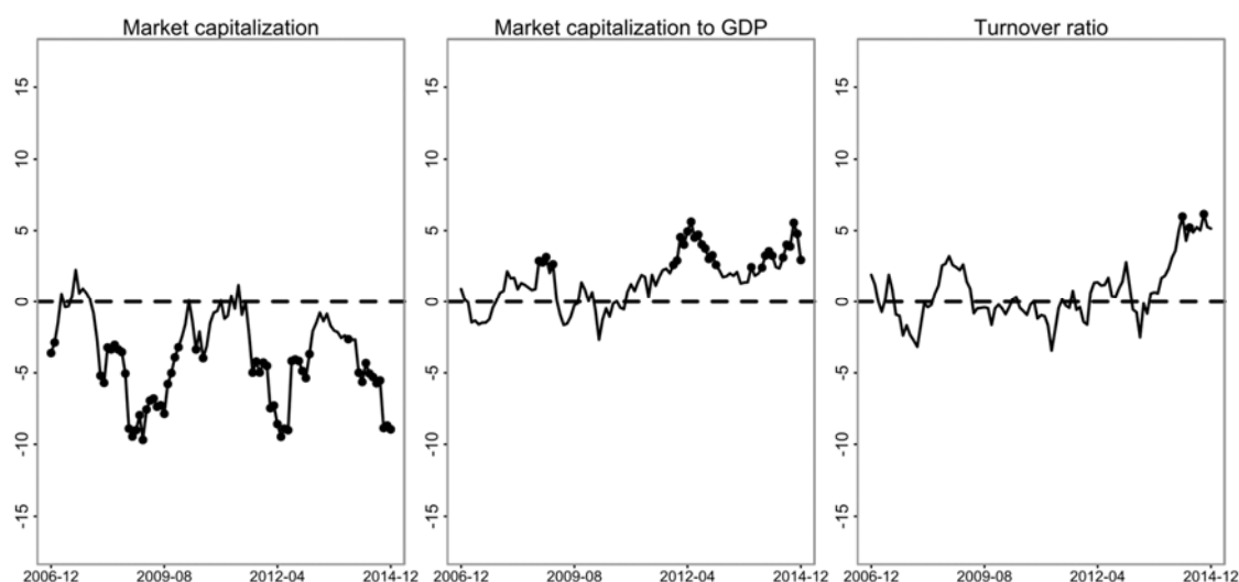
Figure 11. Average direct effects of market capitalization and market liquidity (in-vertex). Note: Bullets denote statistically significant coefficients at the 5% significance level.
