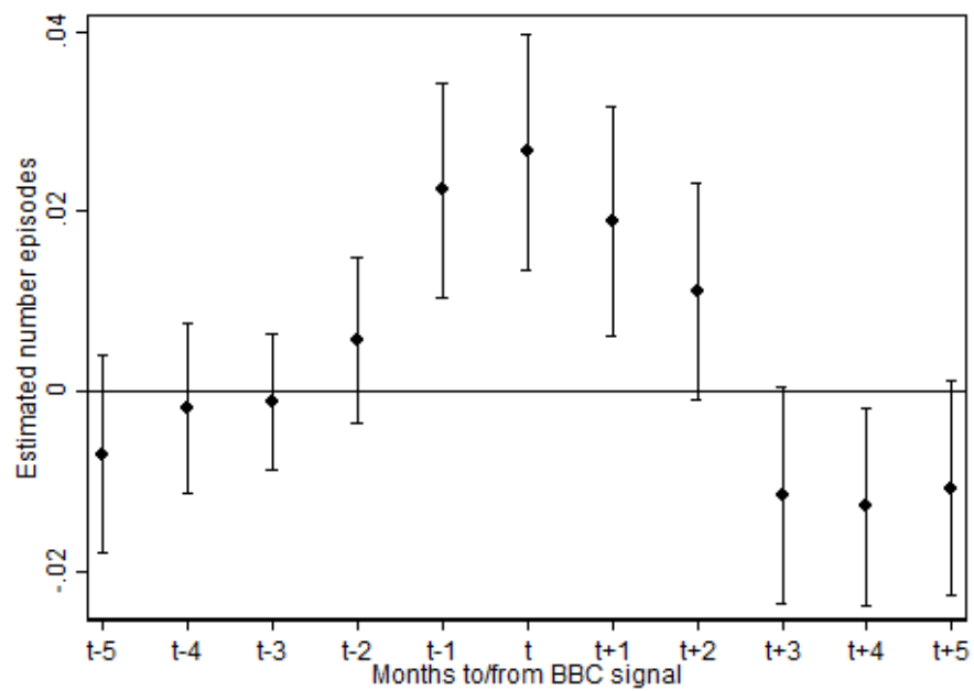
Figure 7: Leads and Lags
