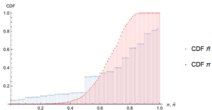
(a) CDF
