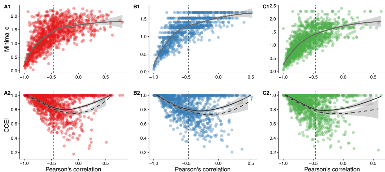
Figure 5: x -axis is Pearson’s correlation between \log(x_2/x_1) and \log(p_2/p_1) . The vertical dashed line indicates the critical value below which Pearson’s correlation is significantly negative (one-tailed test, at 1% level). Solid curves represent LOESS smoothing. Dashed lines in the second row represent LOESS smoothing excluding subjects with CCEI = 1 . Panels: (A) CKMS, (B) CMW, (C) CS.
