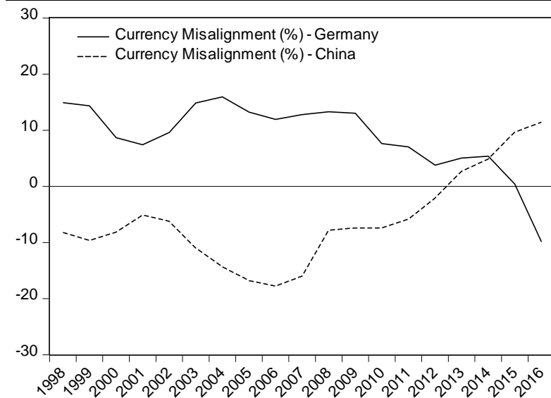
Figure 3: Currency Misalignment
