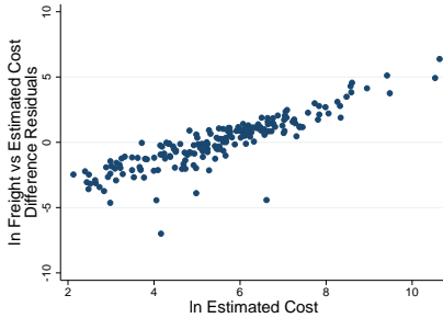
(A) Approximated Error vs Estimated Costs
