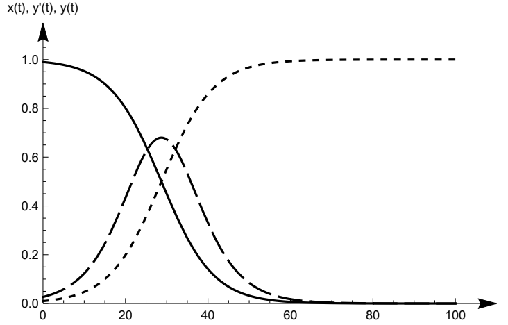
Figure 2: Dynamics in model 1 absent policy intervention: x(t) (solid), \hat{y}(t) (scaled, dashed), and y(t) = (1 - x(t)) (dotted).
