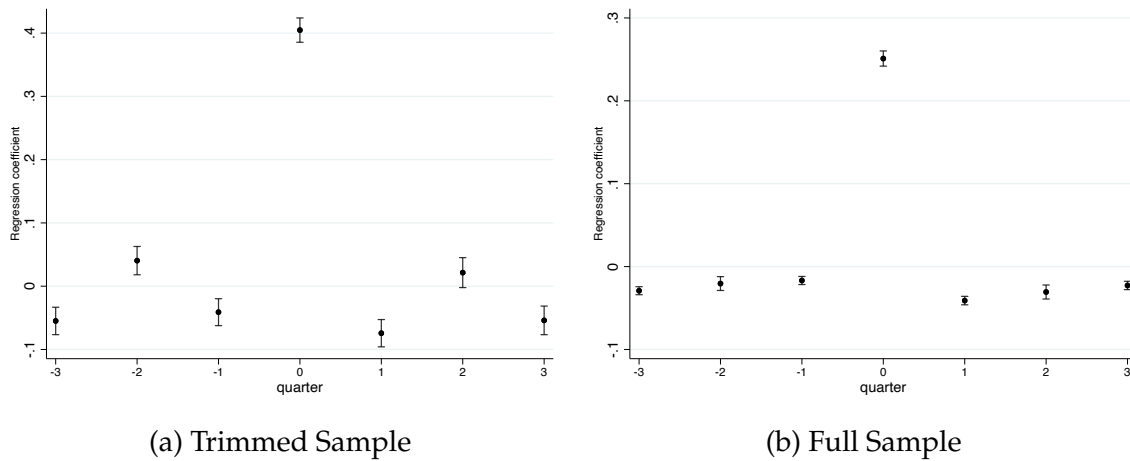
Figure C.5: Cross-correlation
