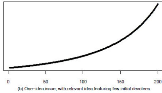
Figure 3: Simulated timelines
