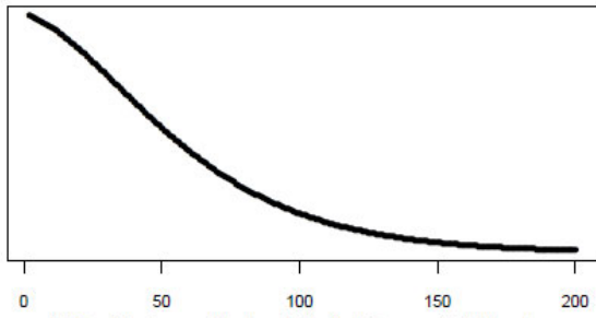
Figure 3: Simulated timelines
