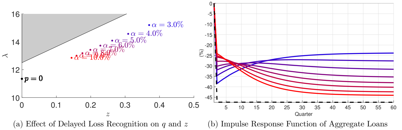
Figure 14: Counterfactual Exercise
