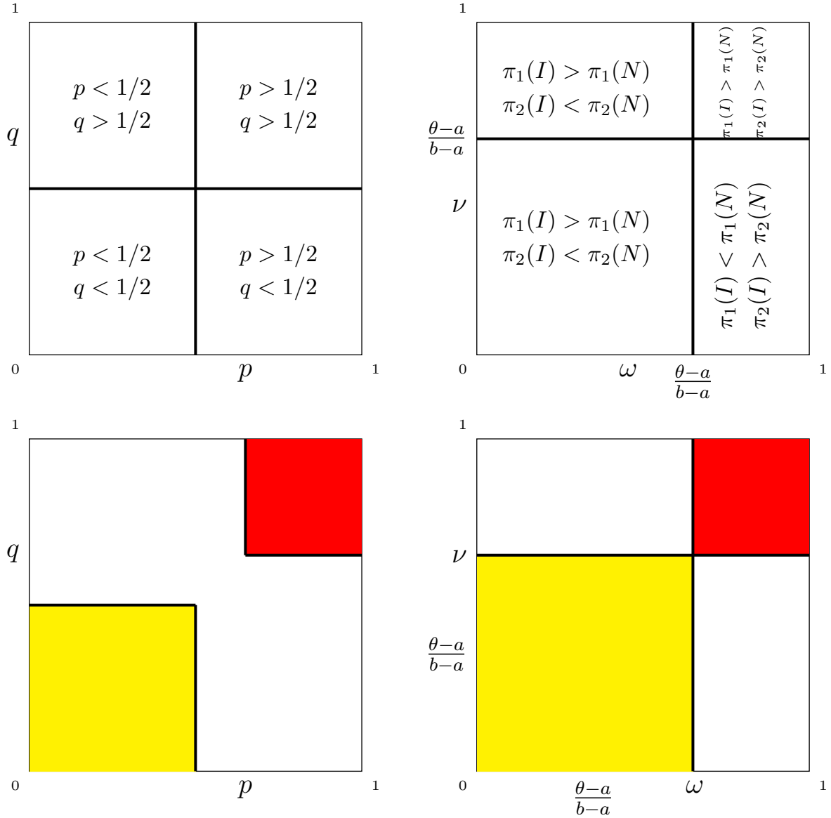
Figure A2: Construction of M -Choice and M -Belief Sets for Games with \theta \in [(a+b)/2, b] . The top panel show partitions of the unit square based on orderings of choice probabilities (left) and expected payoffs (right). There are two M -choice sets for which these orderings match, see the lower-left panel, which can be labeled or colored by the ordering they represent. The colored sets in the lower-right panel show the beliefs that generate the same ordering of expected payoffs as choices of the same color.
