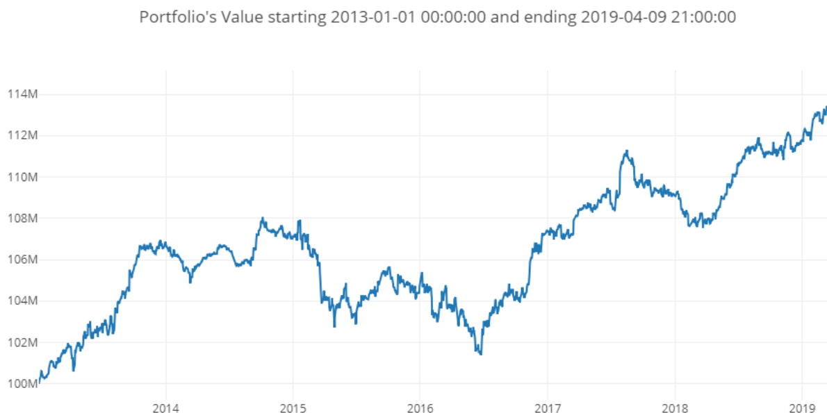
Figure 2: Intraday Strategy (1) cumulative portfolio value
