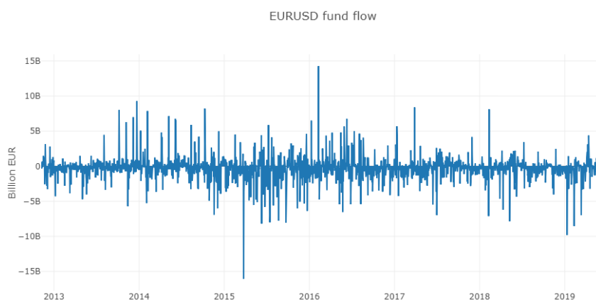
Figure 1: EURUSD Daily Flows
