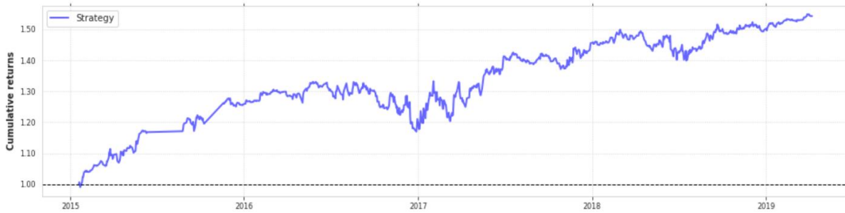
Figure 8: Fund and Corporate Flows Cumulative Returns
