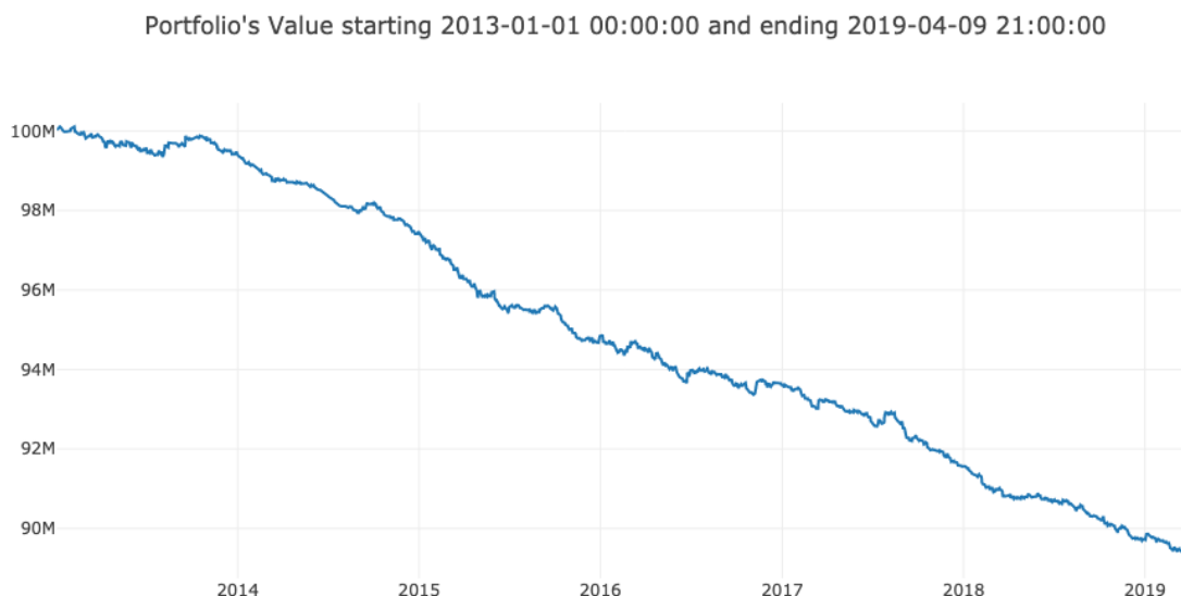
Figure 4. Intraday strategy (3) Funds + Corporate with transaction cost.
