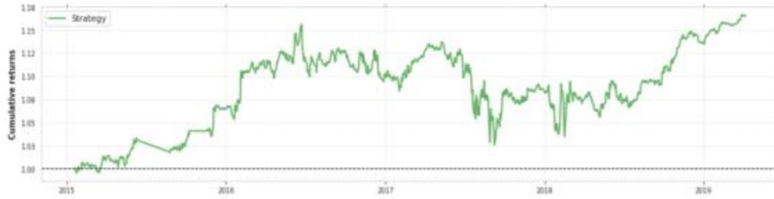
Figure 6: Momentum Signal Cumulative Returns
