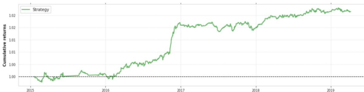
Figure 5. Daily strategy (1) Funds flows only
