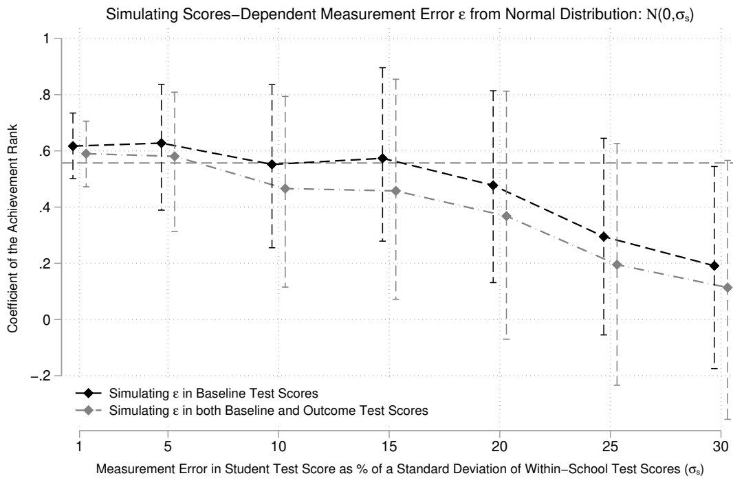
Figure B.2: ESTIMATION OF RANK EFFECTS FROM A SPECIFICATION WITH SIMULATED SCORE-DEPENDENT MEASUREMENT ERROR IN TEST SCORES
