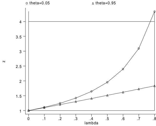
Figure 1: Combinations of \lambda and z ensuring that perfect sorting is locally optimal.
